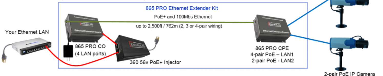
Option 1 – Normal Remote PoE+ use up to 2,500ft
